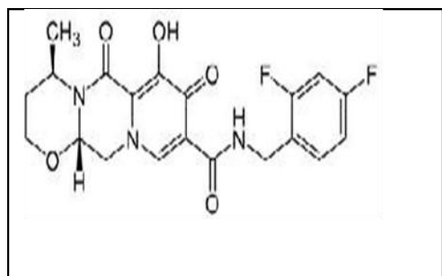
Figure 3: Structure of Dolutagravir
