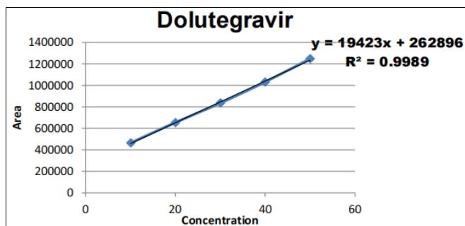
Figure 10: Linearity Graph of Dolutegravir
