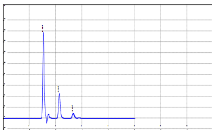
Figure 7: Chromatogram of standard solution of Lamivudine, Tenofovir and Dolutegravir
