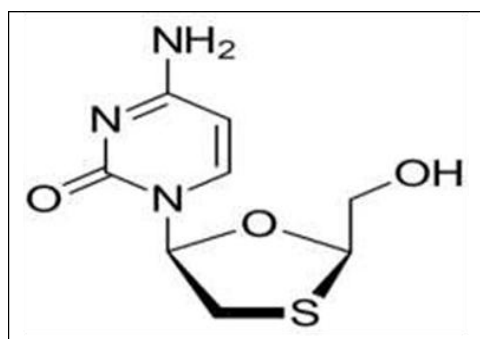
Figure 1: Structure of Lamivudine
