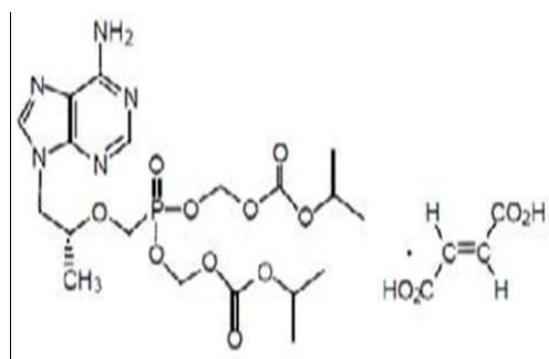
Figure 2 : Structure of Tenofovir Disproxil
