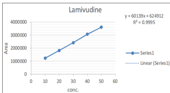
Figure 13: Ruggedness graph for Lamivudine
