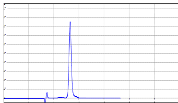
Figure 6: Retention time of Dolutegravir
