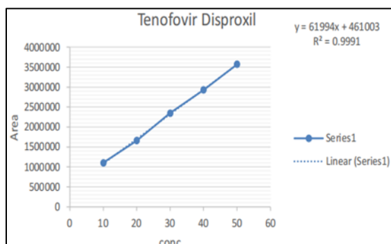
Figure 14: Ruggedness graph for Tenofovir Disproxil
