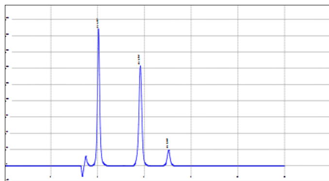
Figure 11: Graph for % Assay of Lamivudine, Tenofovir Disoproxil and Dolutegravir
