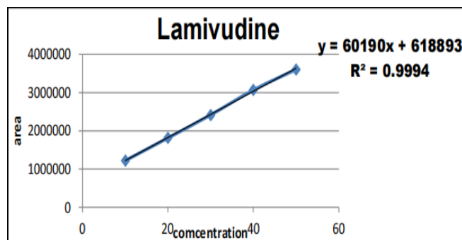
Figure 8: linearity graph for Lamivudine
