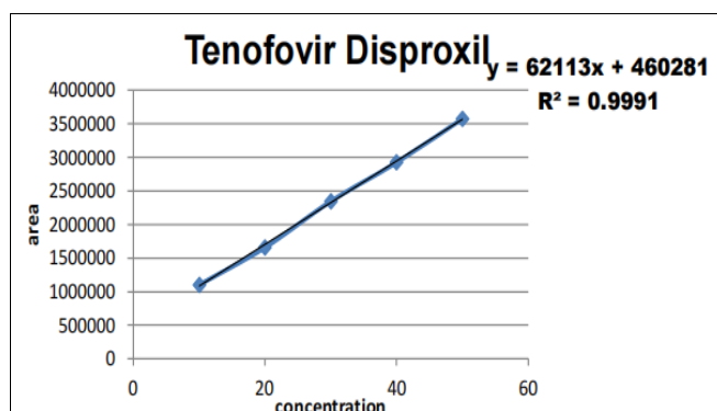
Figure 9: Linearity Graph of Tenofovir Disoproxil
