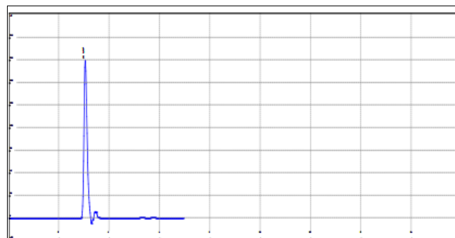
Figure 4 Retention time of Lamivudine
