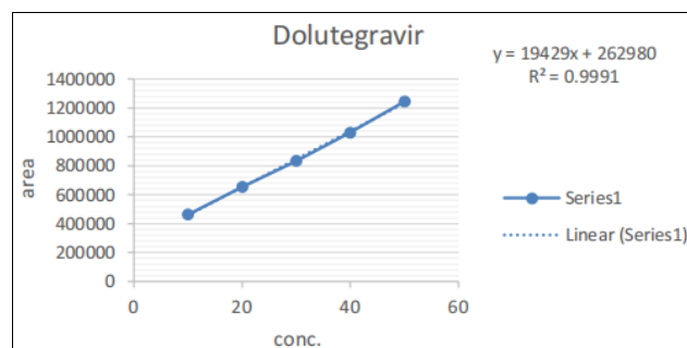
Figure 15: Ruggedness graph for Dolutegravir
